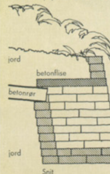
Snit
