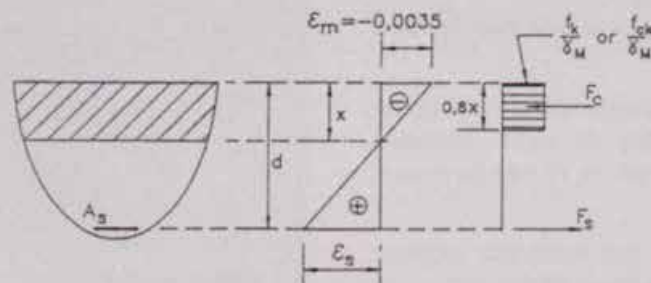
Figure 4.10: Simplified rectangular stress block
