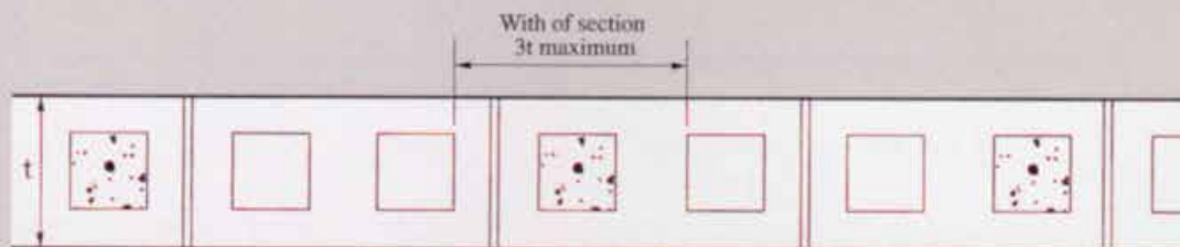
Figure 4.11 : Width of section for members with locally concentrated reinforcement.
