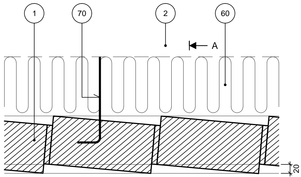
Snit B - B
